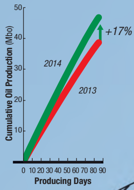
Improving 90-Day Oil Production in the Leonard Shale
